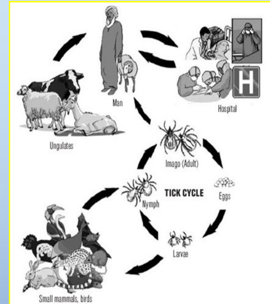
Figure 4. Example of CCHF virus circulation: transmission by the Hyalomma marginatum rufipes ticks. Context: Pierre Nabeth. Crimean-Congo Haemorrhagic Fever Virus In Emerging Viruses in Human Populations (Edward Tabor, editor) Elsevier Science, 2007, (England). Figure-3, p 307.
