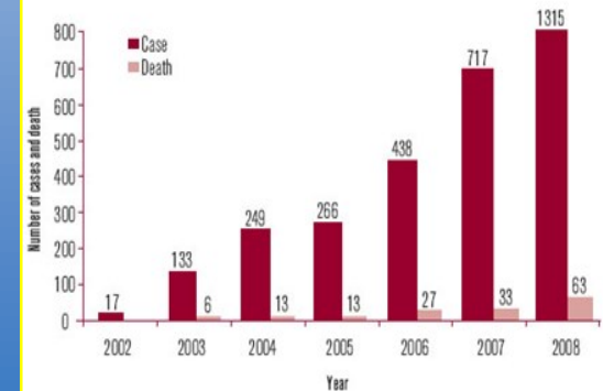
Figure 5. Number of Crimean-Congo hemorrhagic fever cases and deaths in Turkey between 2002-2008. 32
